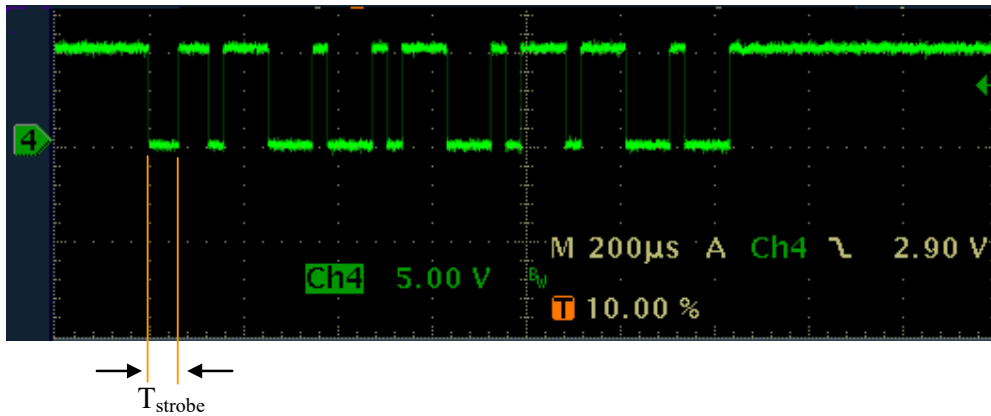
Figure 1.3 – ZACwire™ Transmission
