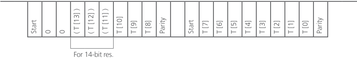
Figure 1.2 – Full ZACwire™ Temperature Transmission from TSic
