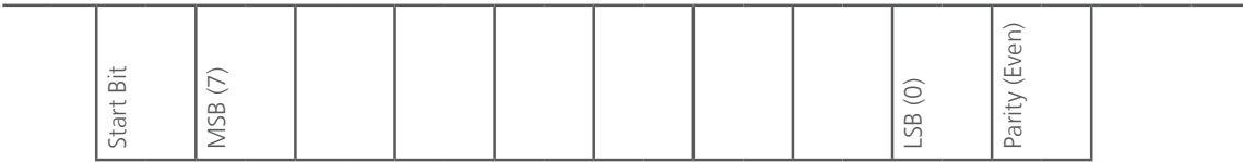
Figure 1.1 – ZACwire™ Transmission Packet
